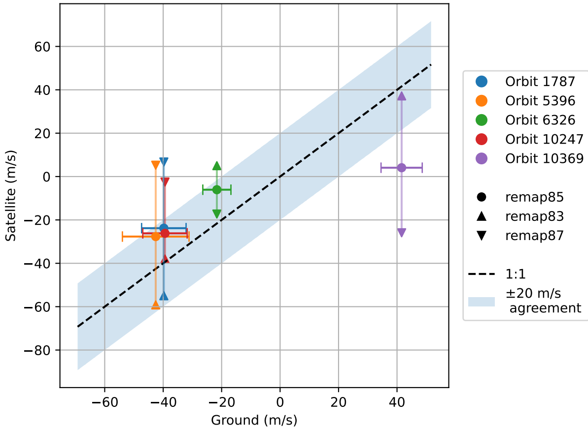
Phase Speed: Ground vs Satellite (83 / 85 / 87)
